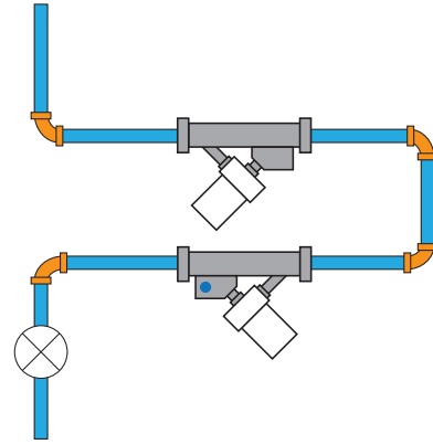
Diagram 18.1 Shows how to fit two pumps in series when there is limited space and applies to all applications of the Shower Power Booster.
