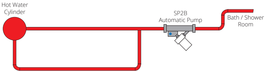
Diagram 22.2 Automatic Pump (SP2B) installed after the return.
