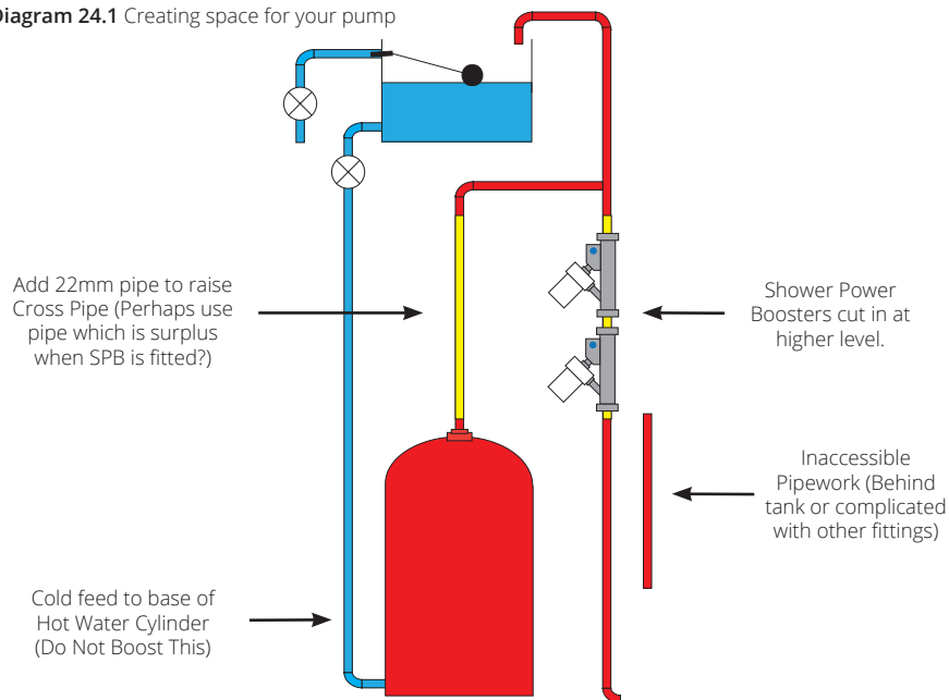
Diagram 24.1 Creating space for your pump
