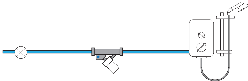
Diagram 18.2 Automatic Pump (SP2B) installed on Mains fed cold to an Electric Shower.
