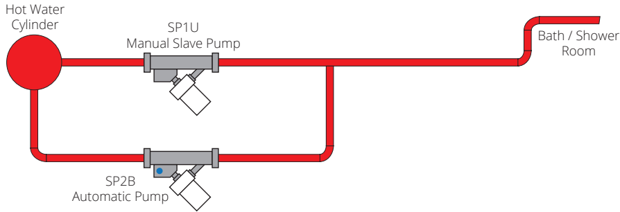
Diagram 22.1 Automatic & Manual Pumps (SP21S) installed on the delivery and return.
